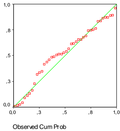
Normal P-P Plot of Regression Sta Dependent Variable: TRANSFER P
