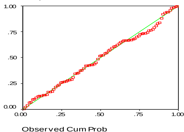
Gambar 4.3 : Grafik Normal P-Plot of Regression Standardized
