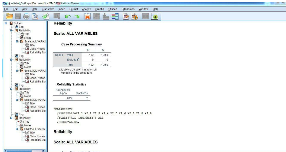
Gambar 2. Uji Reliabelitas
