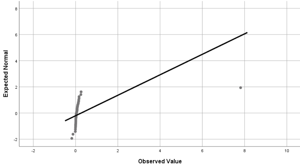
Normal Q-Q Plot of ROE SEBELUM COVID-19
