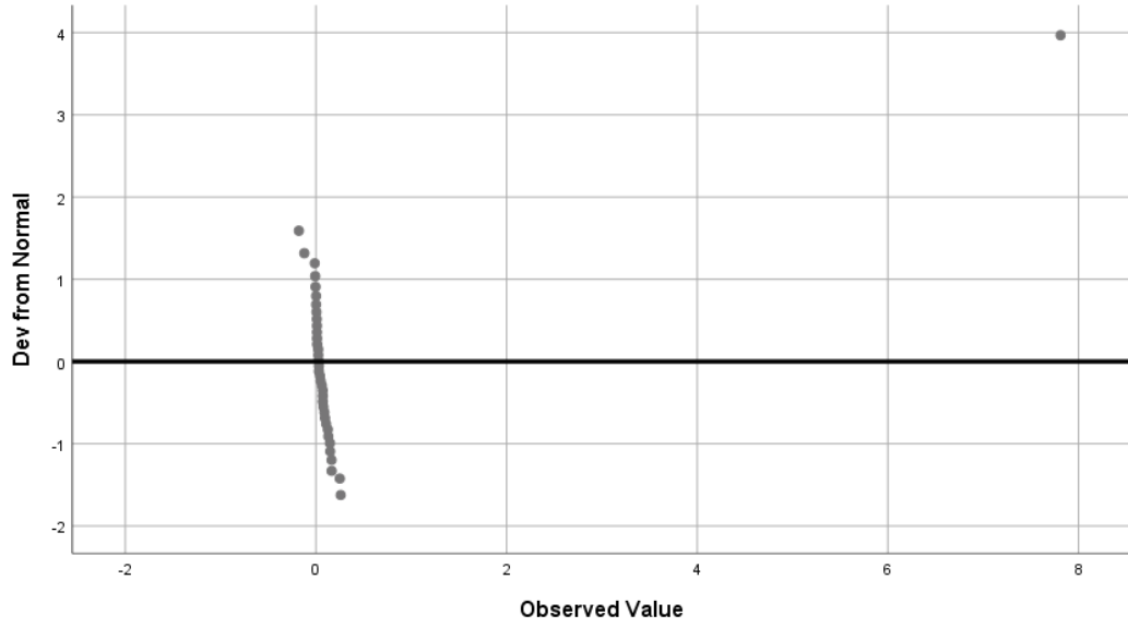
Detrended Normal Q-Q Plot of ROE SEBELUM COVID-19
