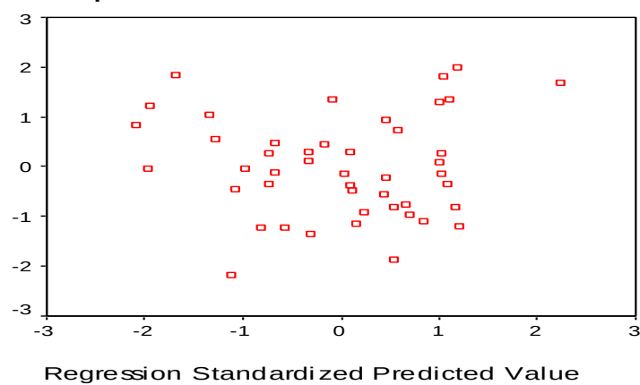
Scatterplot
